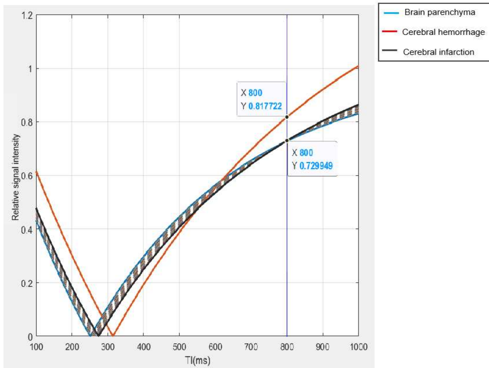
Supplement Figure 2. The changing signals of hemorrhagic, ischemic, and normal brain parenchyma based on inversion time values at 0.23-T MRI.
