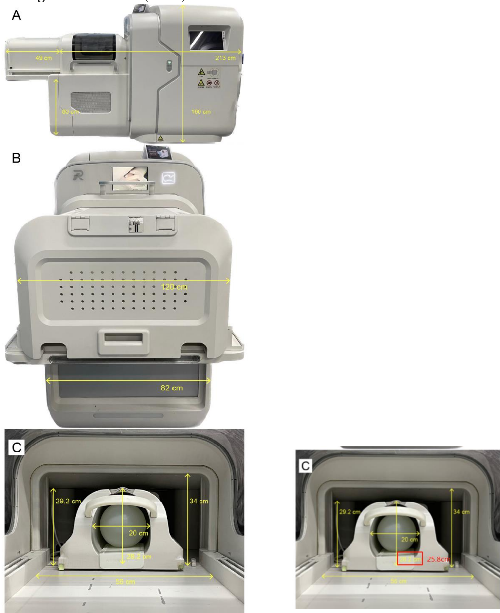
Supplement Figure 1. Low-field (0.23T) MRI device dimensions.
